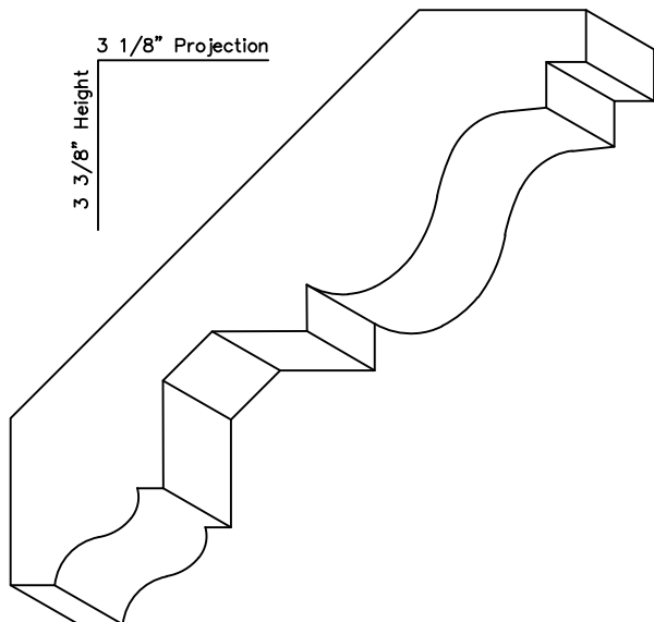
2065 Dentil Crown 13/16" x 3 7/8"
