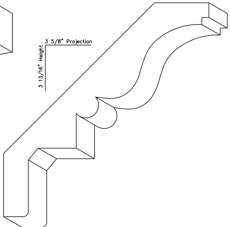
2067 Dentil Crown 1 1/16" x 5 1/4"
